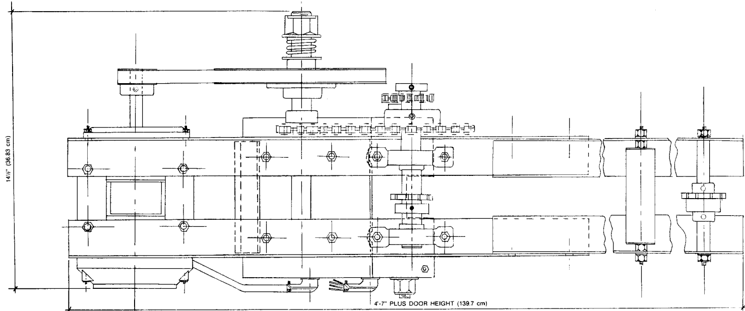
PLAN VIEW (LOOKING FROM THE BOTTOM)
